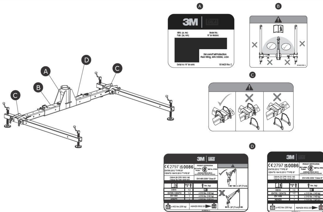
Figure 7- Vörumerkingar
